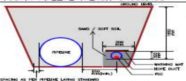
FOC LAYING IN SEPARATE TRENCH
