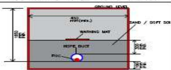
FOC LAYING IN SEPARATE TRENCH
