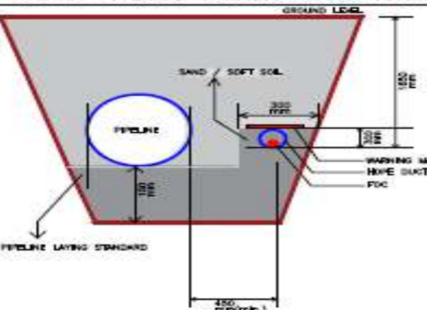
FOC IN PIPELINE TRENCH-ROCKY AREA
